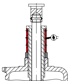
Lock bush
